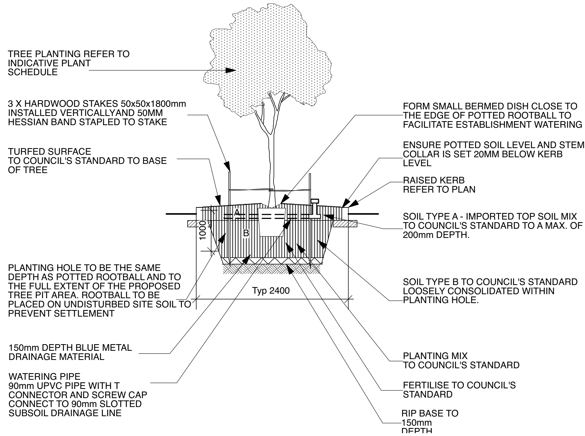
2 Indicative carpark blister tree planting scale 1:50
