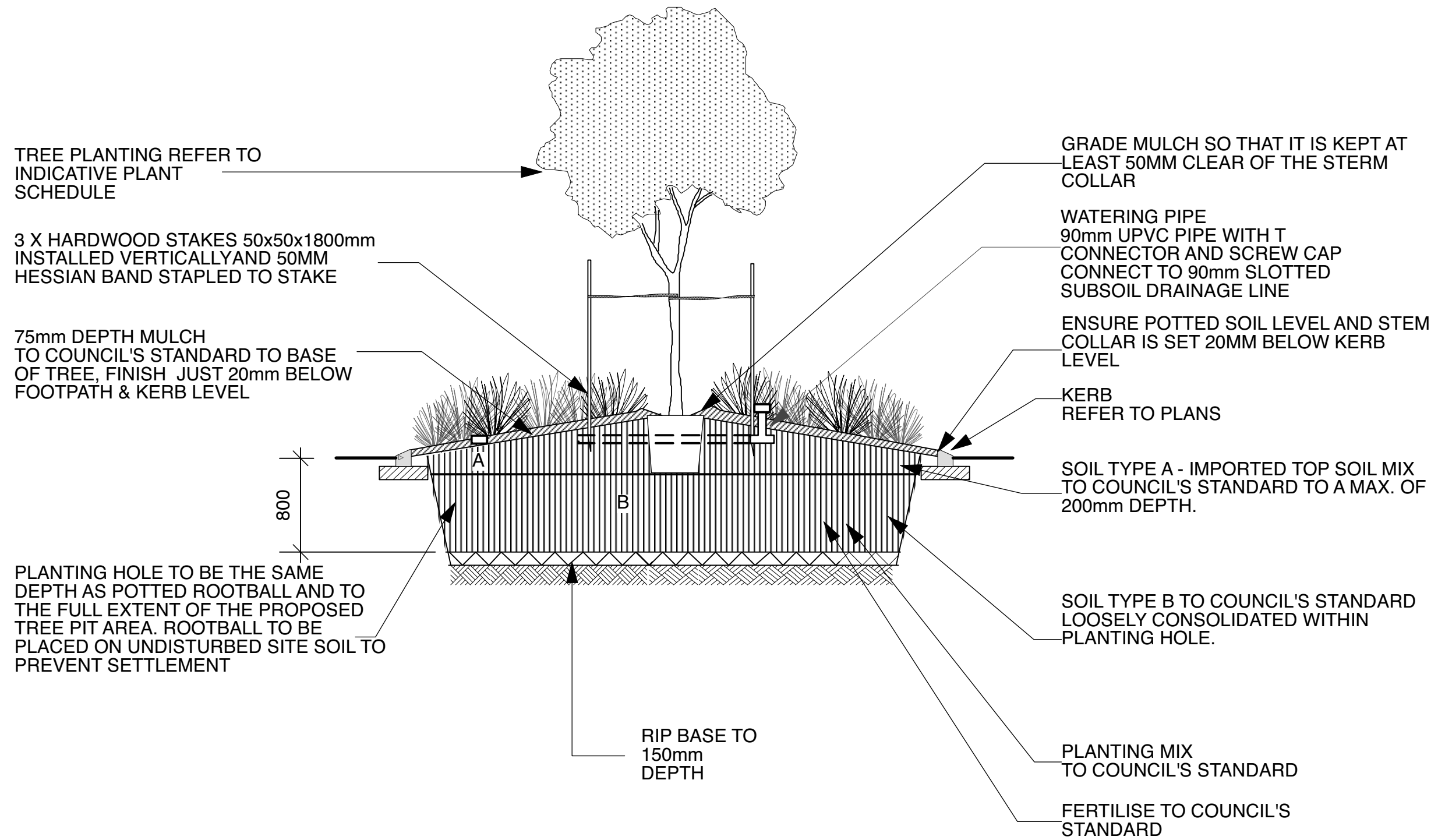
1 Indicative courtyard tree planting scale 1:50
